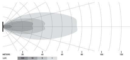
LED Cube KIT 2.7", Flood
