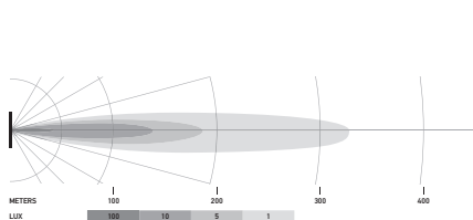
LED Cube KIT 3.2", Spot
