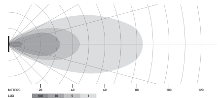
LED Cube KIT 3.2", Flood
